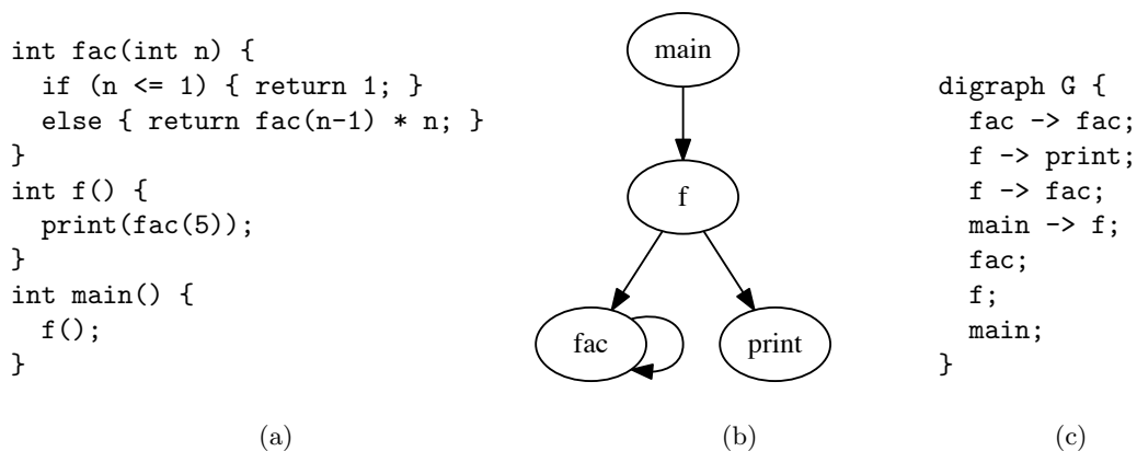
Figure 3: A call graph of a program calculating the factorial of 5. Figure 3c shows the textual representation of the visualized graph expressed in the dot language.
