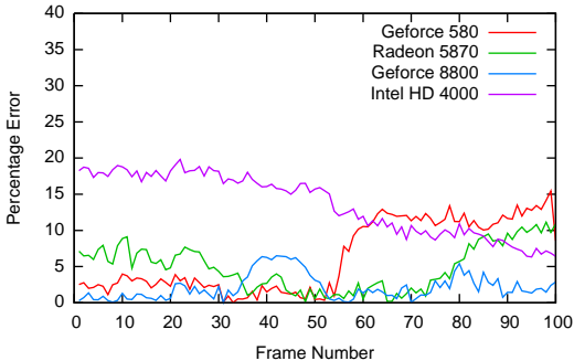
Model to Execution Time Error for Fairy scene
