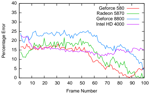
Model to Execution Time Error for Cabin scene
