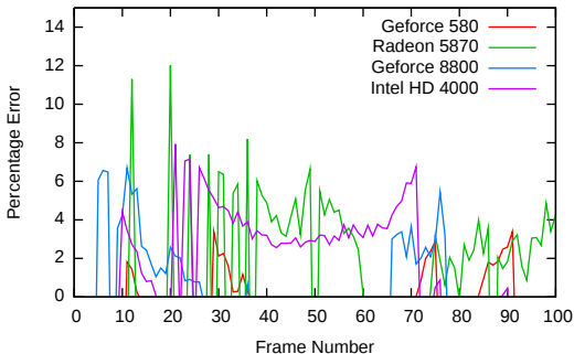
Feedback Model to Execution Time Error for Cabin scene
