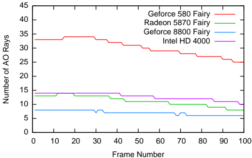
Number of AO Rays Parameter Auto-tuned for Fairy scene
