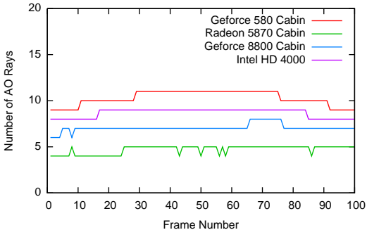
Number of AO Rays Parameter Auto-tuned for Cabin scene
