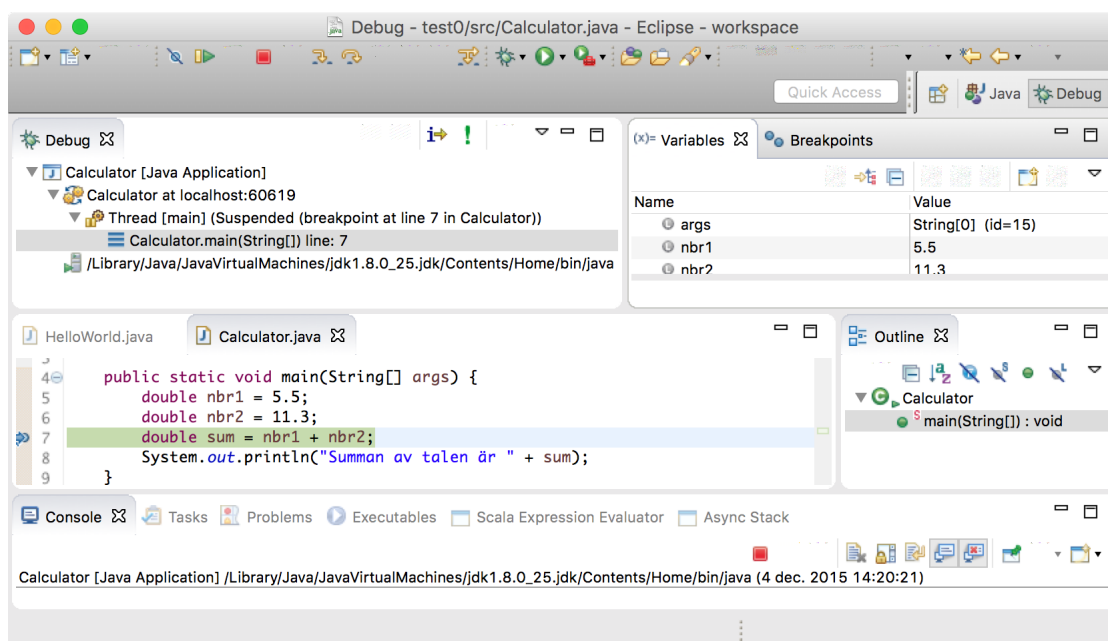
Figur 2: Eclipse-fönster, debug
