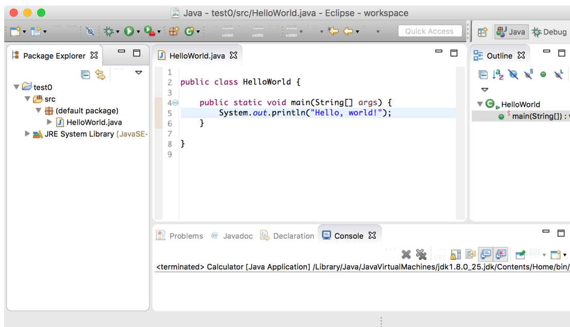
Figur 1: Eclipse-fönster, Java
