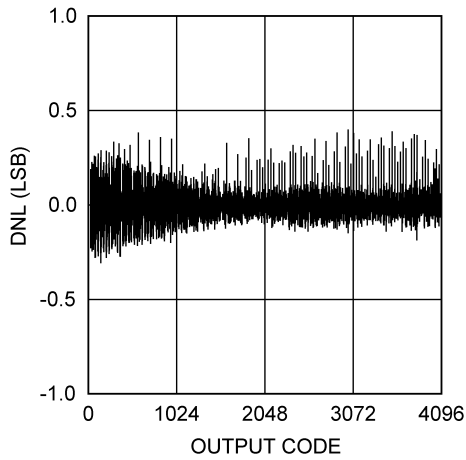
ADCS7476 DNL
