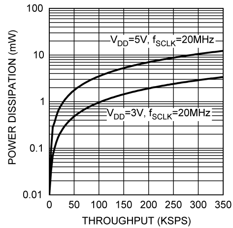
FIGURE 12. Maximum Power Consumption vs. Throughput
