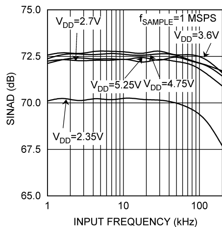
ADCS7476 SINAD vs. Input Frequency, 1 MSPS
