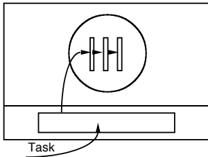
Task pipeline
