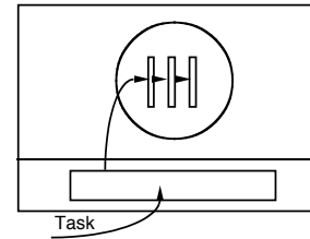
Task pipeline
