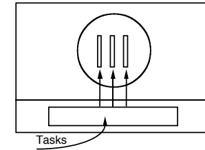
Multiple tasks
